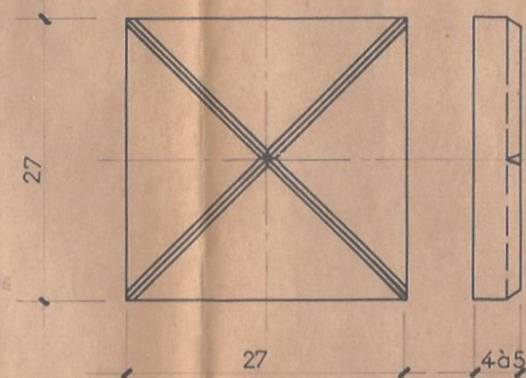
BRIQUE RAINUREE
